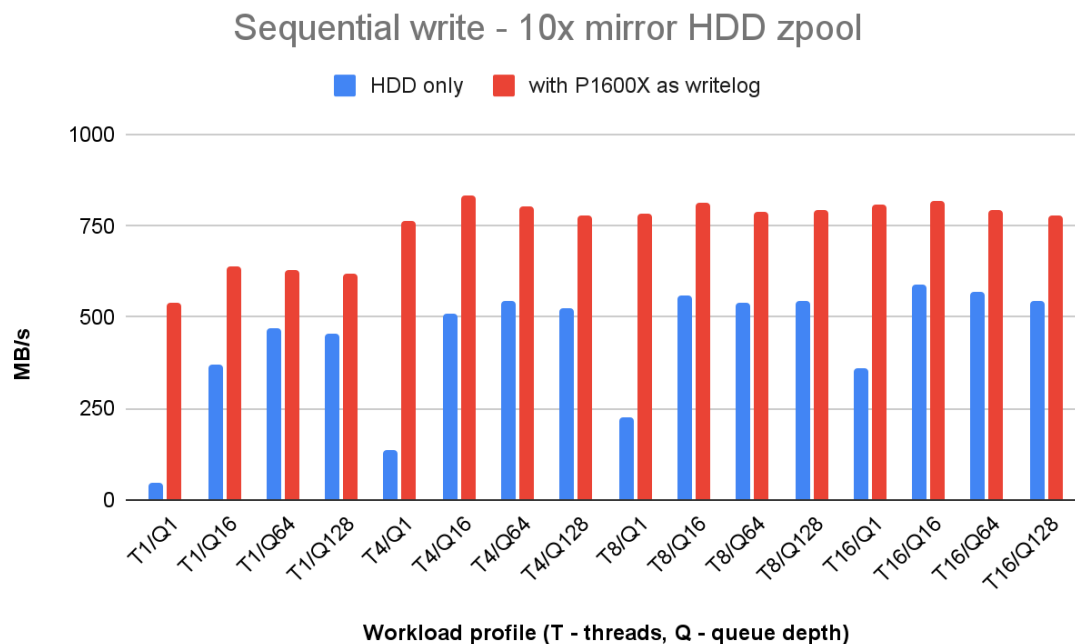
Fig. 13. Sequential write performance of a 10x mirror HDD zpool, with and w/o writelog.
