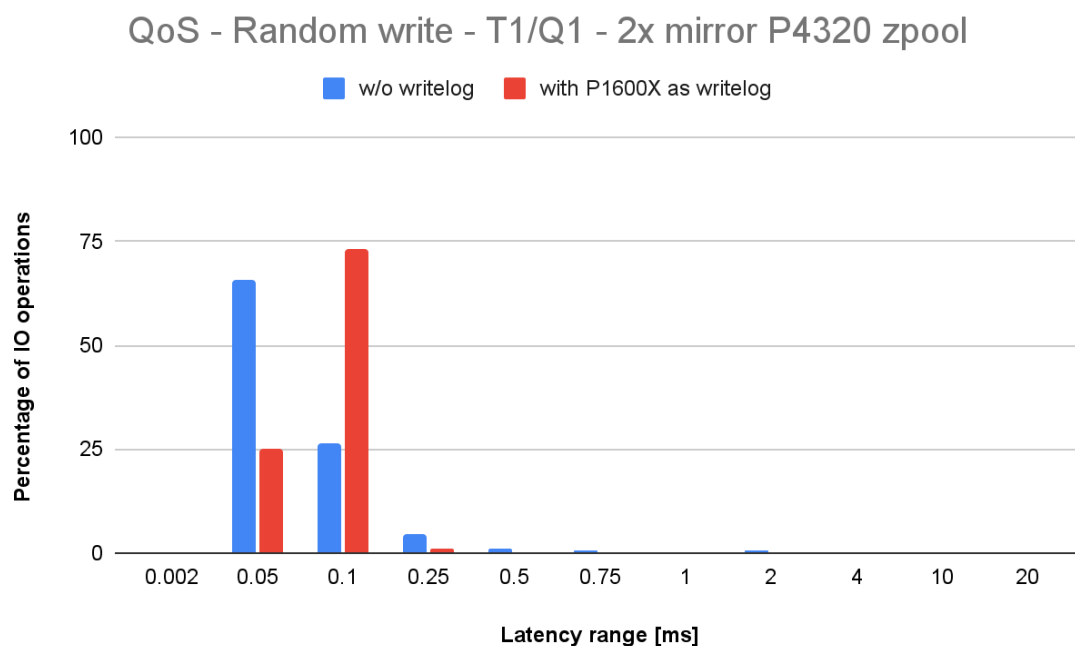
Fig. 23. Latency distribution for a random write test, done on a 2x 2-way mirror SSD zpool (T1/Q1), with and without writelog.
