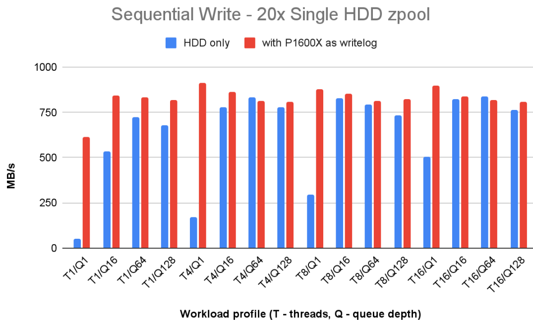
Fig. 19. Sequential write performance of a 20x single HDD zpool, with and w/o writelog.
